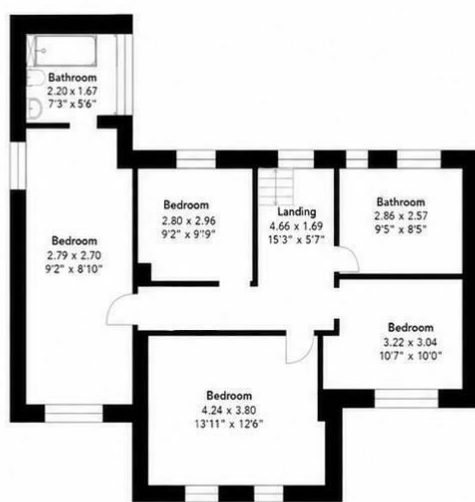
Floor 1 63.1 sq.m
